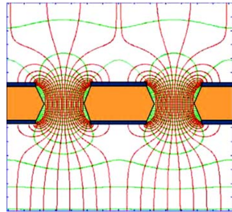
Fig. 3. Cross-section of a GEM showing electric field lines passing through the holes creating regions of high E-field density
