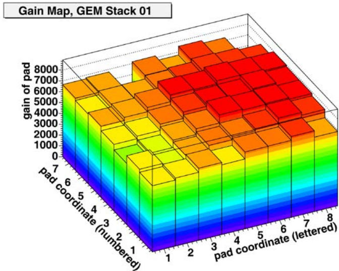
Fig. 8. Gain Map of a triple GEM stack presently installed in the HBD
