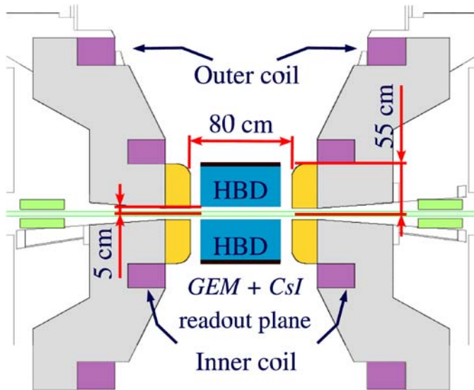
Fig. 1. Layout of the inner part of the PHENIX detector showing the location of the HBD and the inner coil
