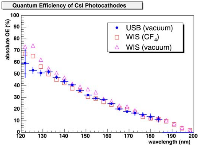
Fig. 7. Quantum efficiency of small gold coated photocathodes plotted as a function of wavelength (measured at BNL)
