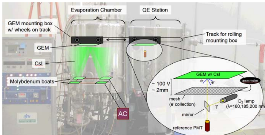
Fig. 6. A picture of the evaporator and quantum efficiency station overlaid with a schematic drawing of the inside of the vessel. The transport box can roll back and forth between the two stations. Highlighted in the lower right is the quantum efficiency station
