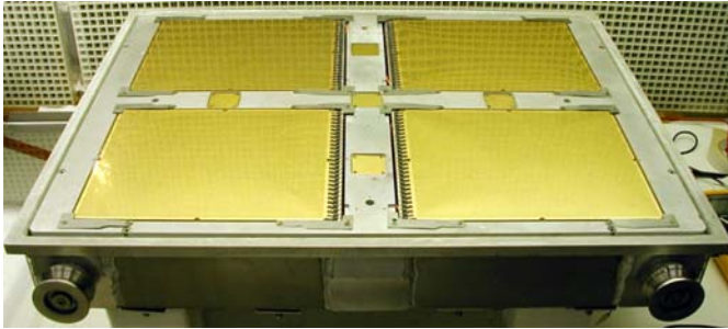
Fig. 5. The transport box which holds the 4 GEMs and 5 smaller, gold-coated photocathodes
