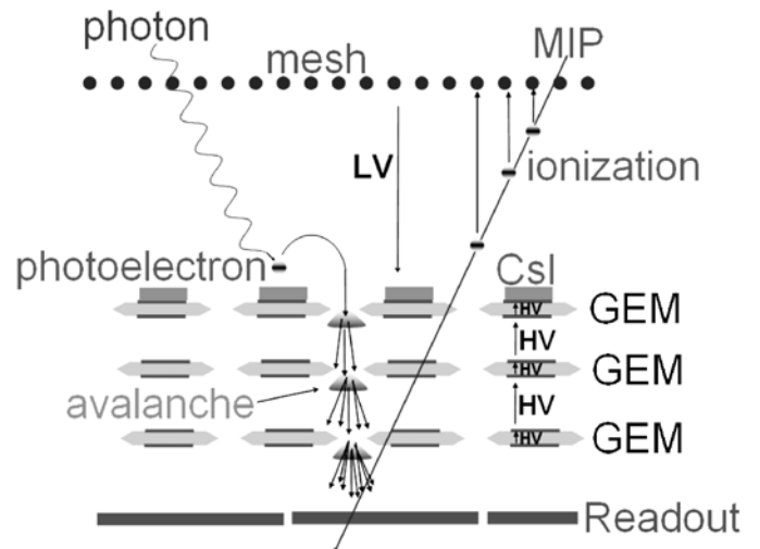
Fig. 4. The schematic cross-section of a triple GEM stack. The top GEM has a \sim 300 nm coating of CsI. Čerenkov-induced photoelectrons are accelerated through the holes while ionization electrons from MIPs are “swept” upwards towards the wire mesh (not to scale)
