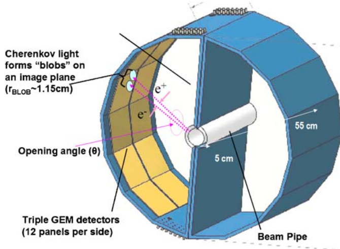
Fig. 2. 3-D depiction of the HBD
